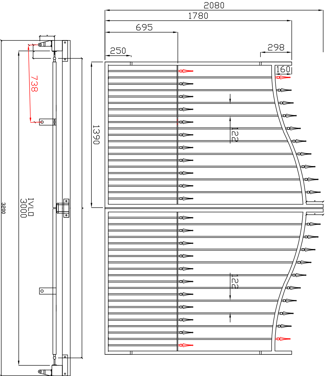
ARCH TOP 3000 X 1780/2080
